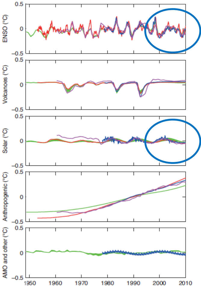
ESTIMATED CONTRIBUTION TO GLOBAL TEMPERATURE (FROM CLIMATE MODELS)
