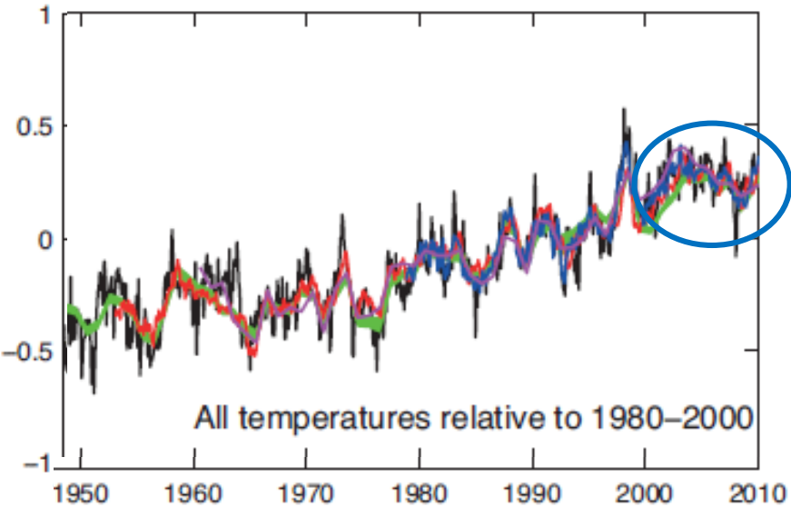
OBSERVED GLOBAL SURFACE TEMPERATURE ANOMALY °C relative to 1980-2000 average
